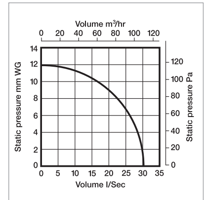
Performance - SF200
