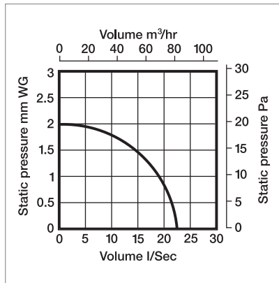
Performance - SF100
