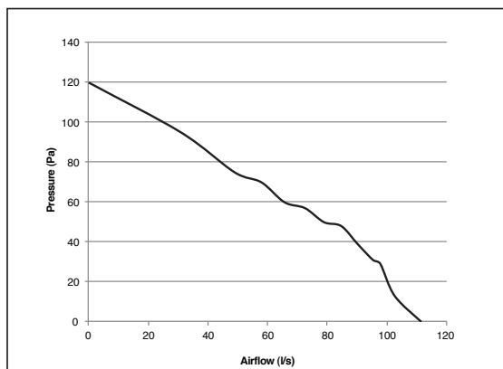
Performance - SF150
