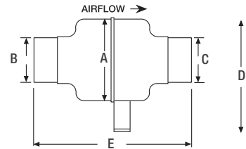
Dimensions - SF200
