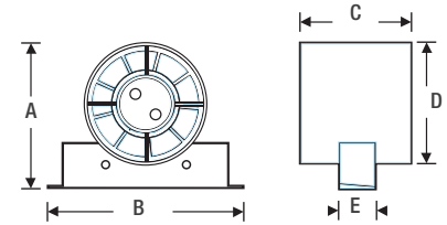
Dimensions - SF100/SF125
